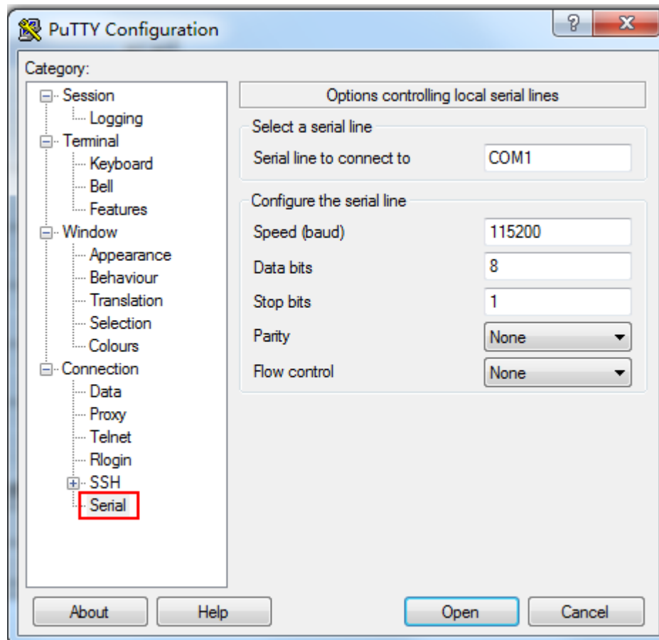
图 8-14 PuTTY Configuration - Serial
